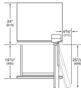
DIMENSIONS WILL VARY WITH PANEL THICKNESS
